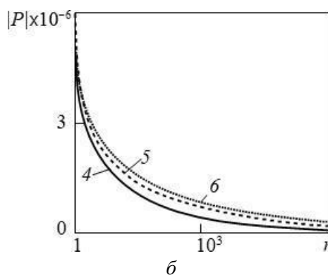
Fig. 4. The pressure dependencies on the radial coordinate for different times. The code for the lines:
